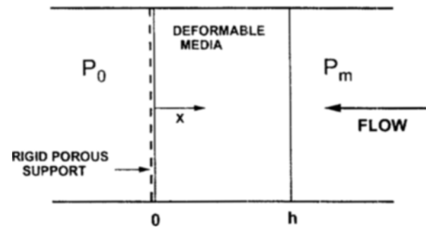
Fig. 2. Planar geometry of the porous media.
