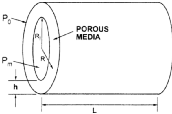
Fig. 1. Cylindrical geometry of the porous media.
